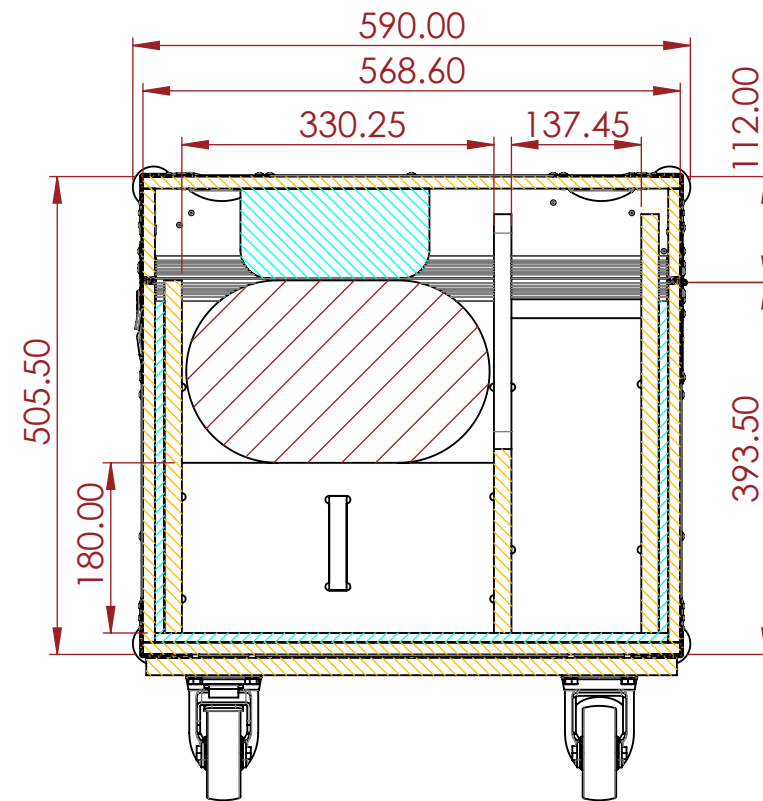
SECTION B-B
