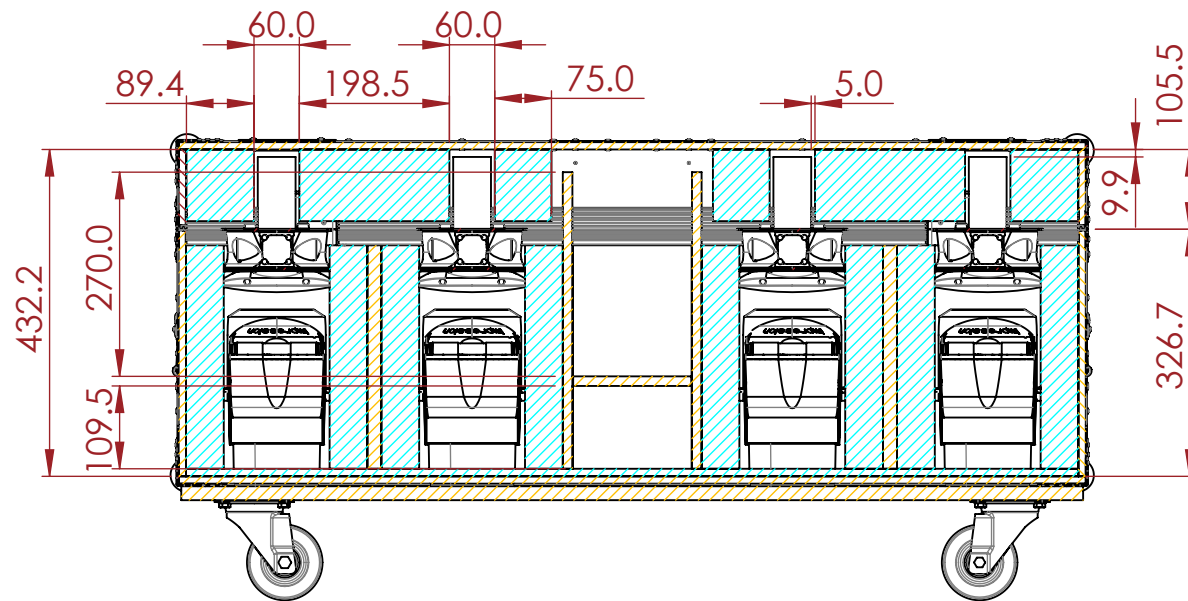
SECTION B-B
